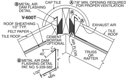
V-600T - \"S\" Tile Application (W/Air Dam Flashing Detail)
