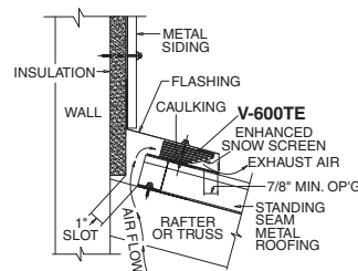
V-600TE Standing Seam Roof to Wall
