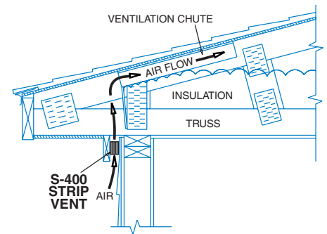
Engineered Truss
