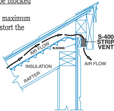
Shed Roof
