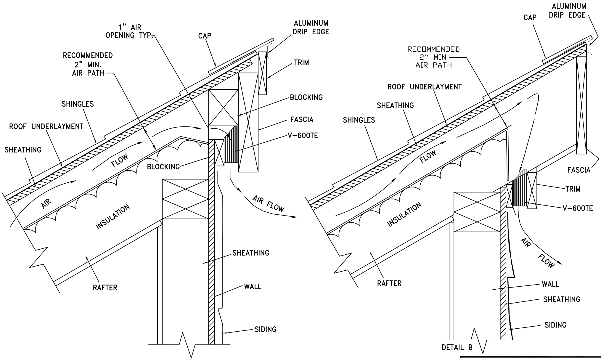
DETAIL A
