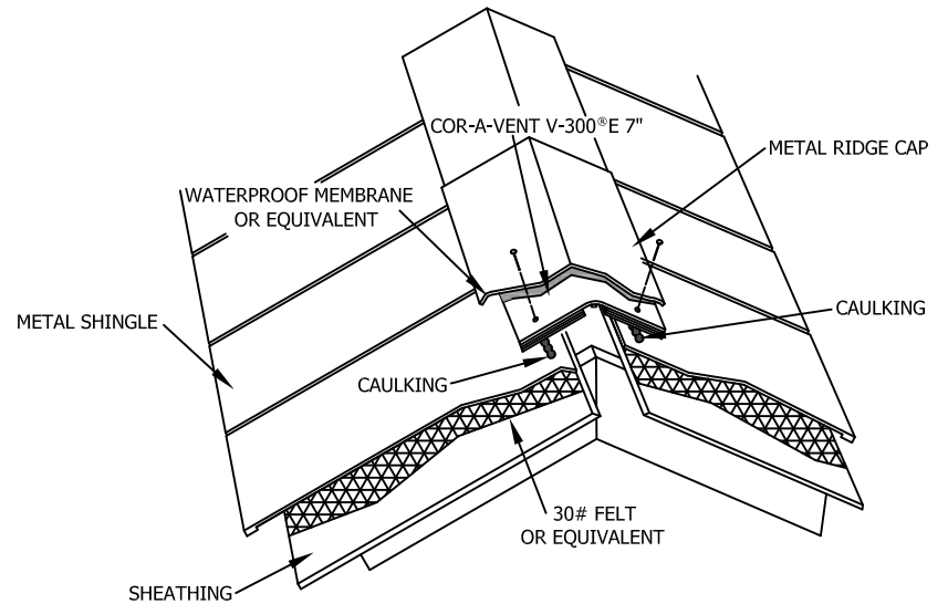
PERSPECTIVE VIEW METAL SHINGLE APPLICATION
