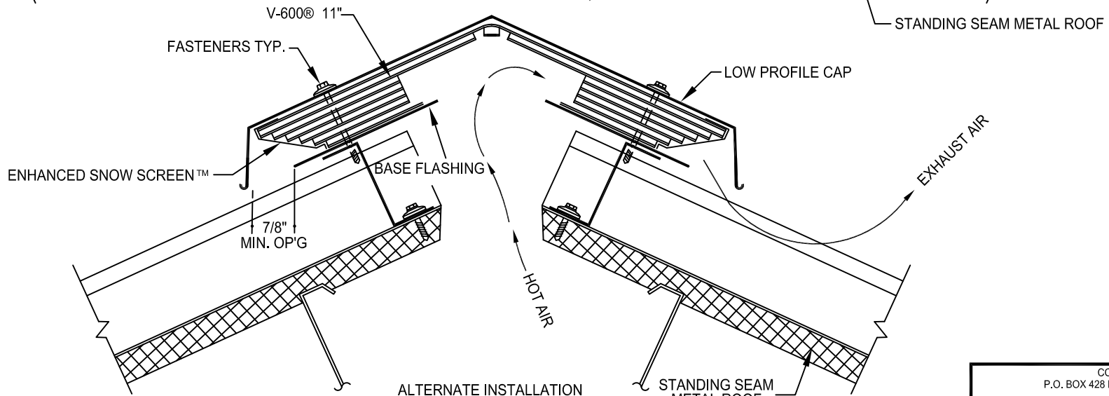
ALTERNATE INSTALLATION SUBSTITUTED V-600@ E 11" FOR ADDED PROTECTION AGAINST SNOW INFILTRATION
